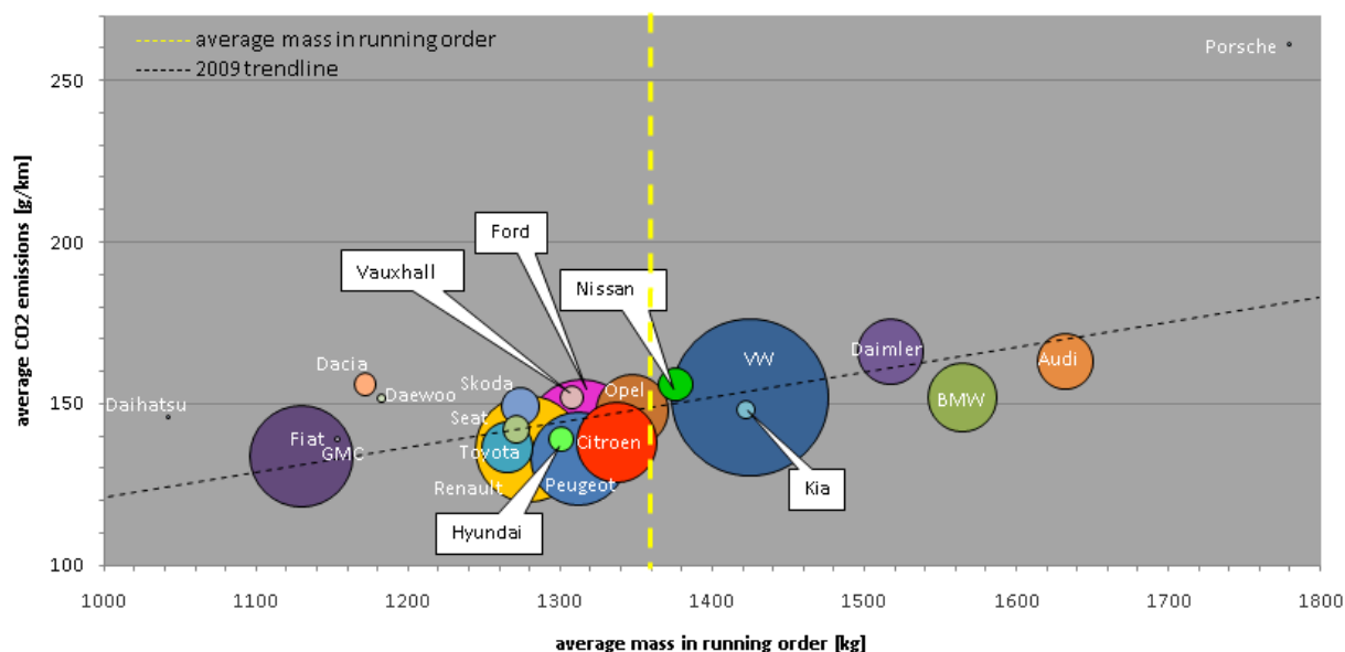
Figure 43 Relationship of the chosen parameter with the CO 2 value.
